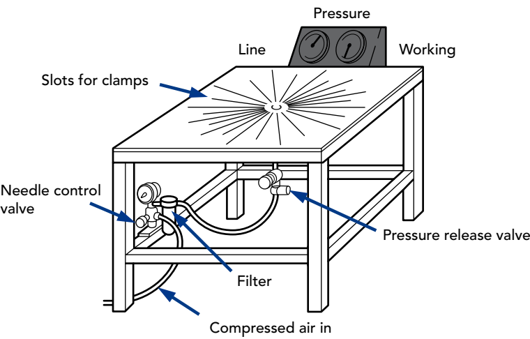
Figure 7 Typical blowing table
