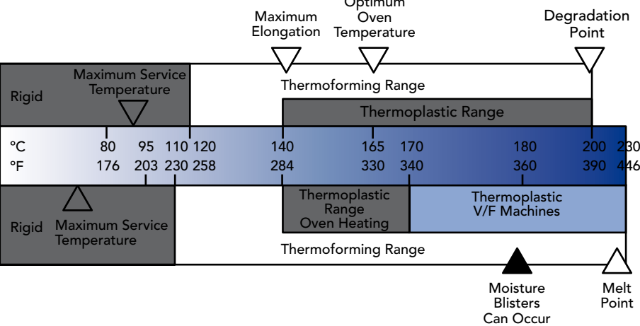
Figure 4 Heating Perspex® – transition stages
