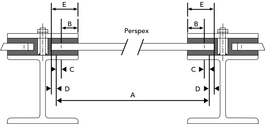
Figure 17 Mounting details for Perspex® glazing
